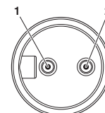
Pin assignment, plug, 7/8"-16UNF, 2-pos., view of male side
