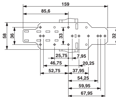
Dimensioned drawing
