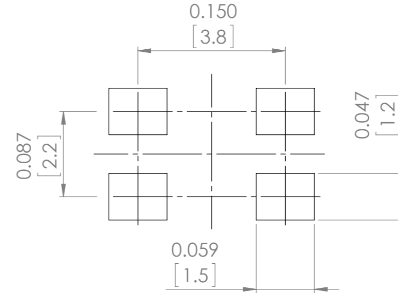
Example for Solder Pattern
